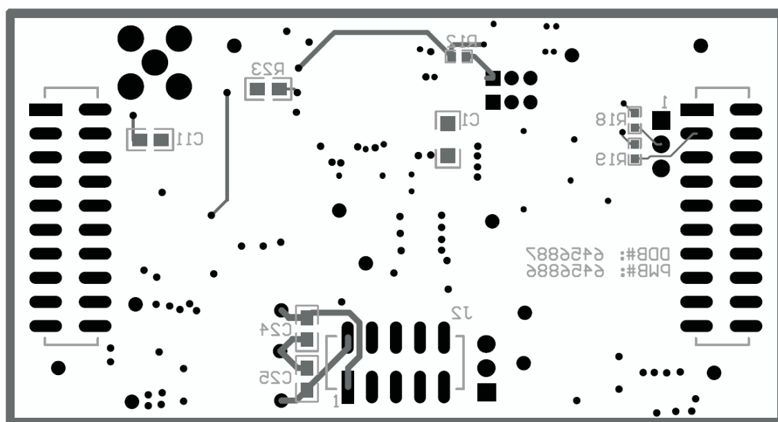
Figure 5. Bottom - Layer 4
